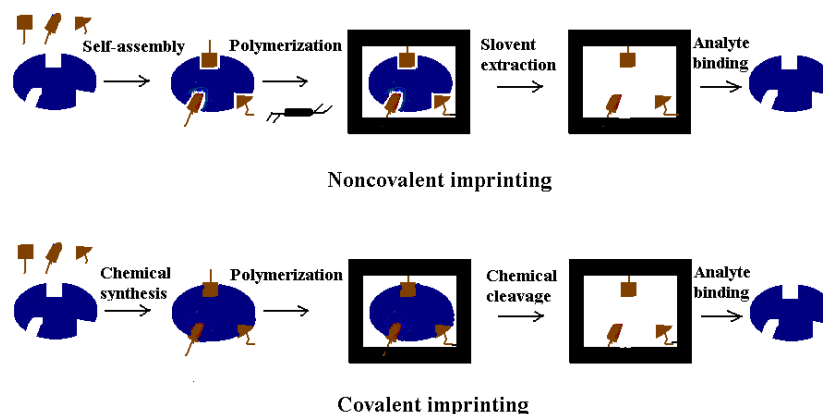
Fig. 3. Schematic illustration of the preparation of molecularly imprinted polymers. Reprinted from ref. [86] with permission from Authors
