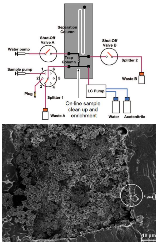
Fig. 5. SPE trap column as a chip design with the SEM image of hydrophobic polymethacrylate monolith covalent attachment to the channel surface. Reprinted from ref. [96] with permission from American Chemical Society
