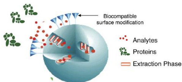
Fig. 2. Schematic illustration of restricted access sorbent. Reprinted from ref. [71] with permission from Springer
