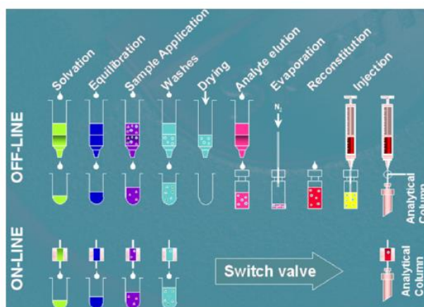
Fig. 1. Schematic illustration of off-line and on-line SPE methodology. Reprinted from ref. [37] with permission from Elsevier
