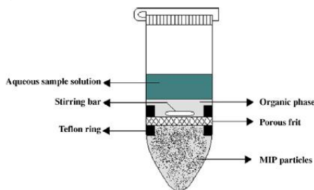
Fig. 4. Schematic illustration of the solvent extraction-molecularly imprinted solid phase extraction (SE-MISPE) cartridge. Reprinted from ref. [80] with permission from Elsevier
